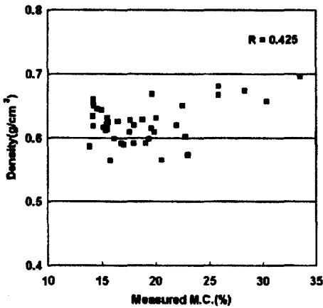
Fig. 11. Density deviation with moisture content.
