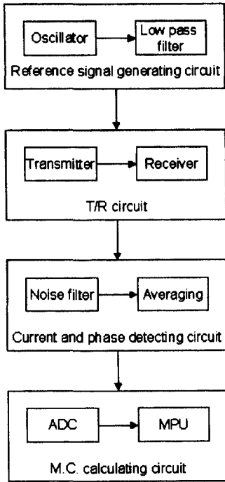
Fig. 7. The block diagram of system for moisture meter.
