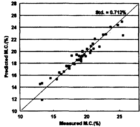
Fig. 8. Validation of calibration model for measuring M.C. of rough rice.
