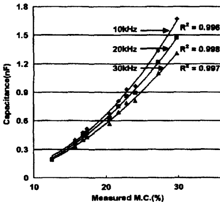
Fig. 5. Capacitance with moisture content.
