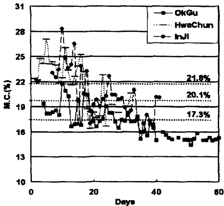
Fig. 1. Distribution of MC with days.
