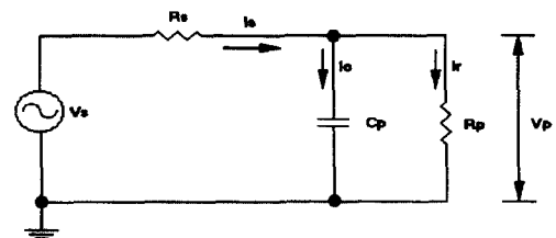
Fig. 3. Basic circuit of the capacitance moisture meter.
