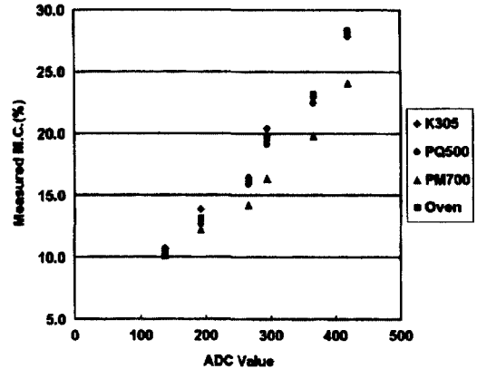
Fig. 9. Calibration model for measuring moisture content of rough rice.
