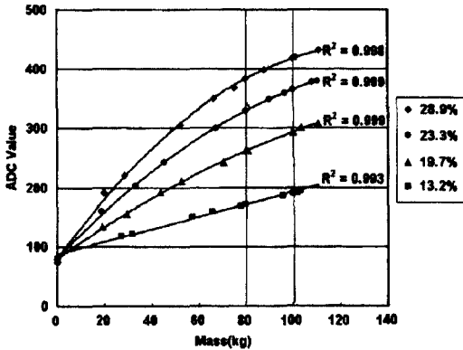
Fig. 10. ADC variation with mass of rough rice.
