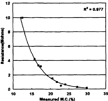
Fig. 6. Resistance with moisture content.
