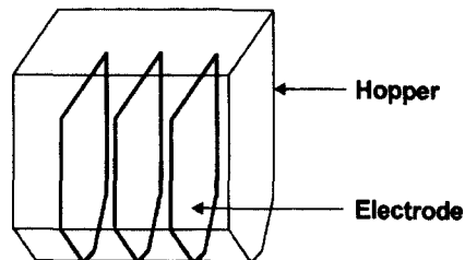
Fig. 4. Structure of hopper and arrangement of electrodes.
